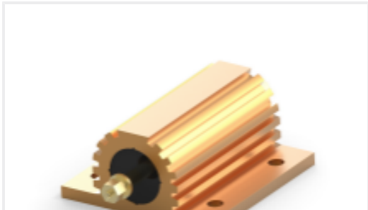
TE Part #4-2176732-9 HSC150S 1K0 5% Screw Terminal
