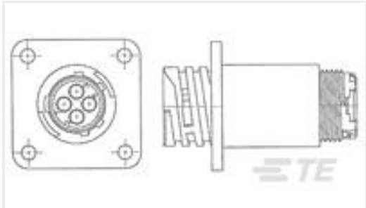
TE Part #1977876-1 SLD CPC RCPT ASY,11-4,STD SEX, UV RESIST
