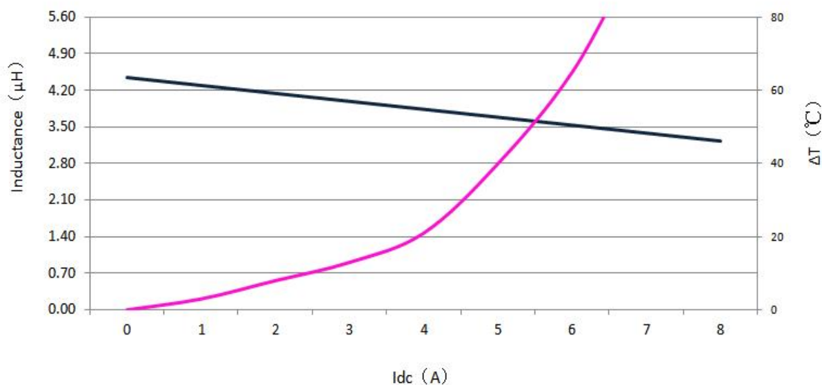
DC Current Curve
