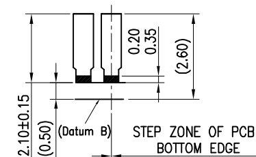
DETAIL F SCALE 8:1
