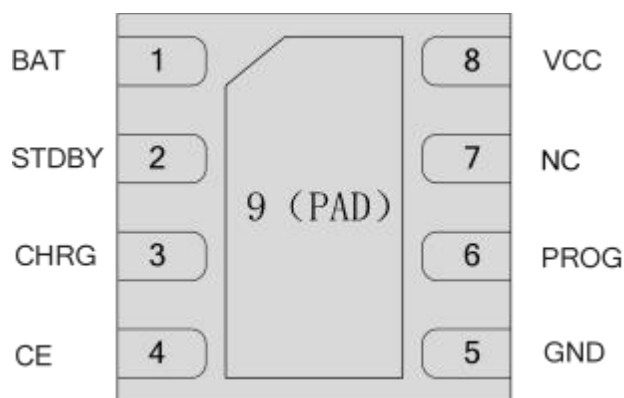
DFN3×3_8L
