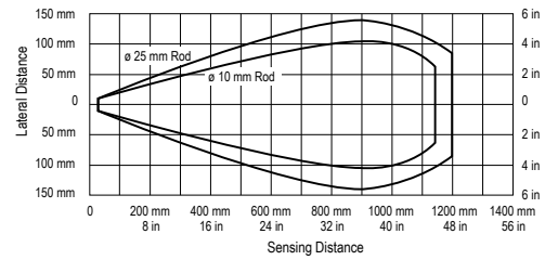
Effective Beam with Rod Target (Typical)
