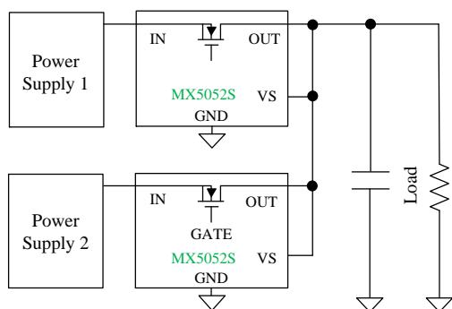
OR-ing With internal MOSFETs
