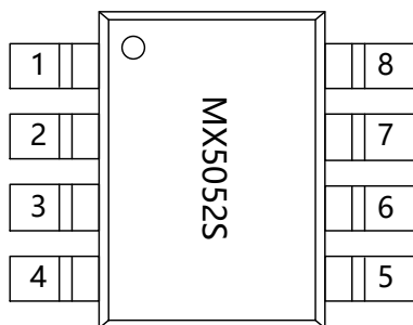
Pin information
