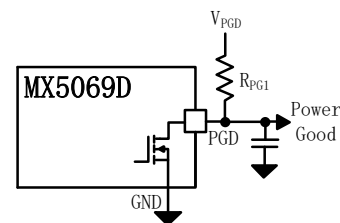
a) Delay Rising Edge Only
