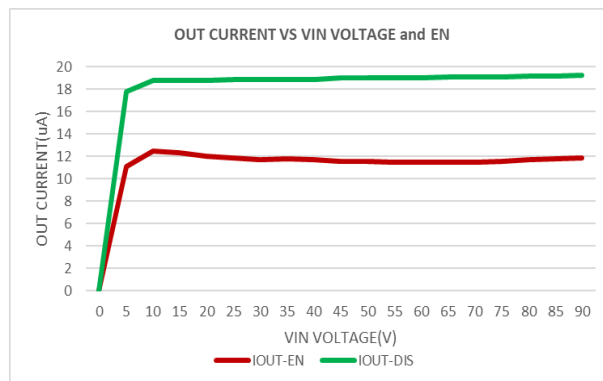
OUT current vs VIN voltage
