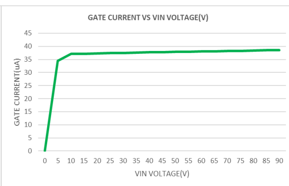
GATE current vs VIN voltage
