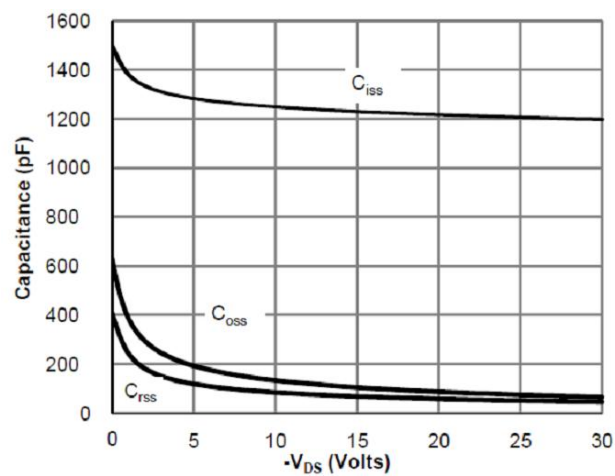
Figure 7. Capacitance Characteristics
