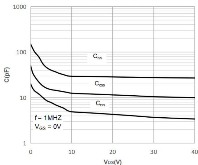
Figure 6: Capacitance Characteristics
