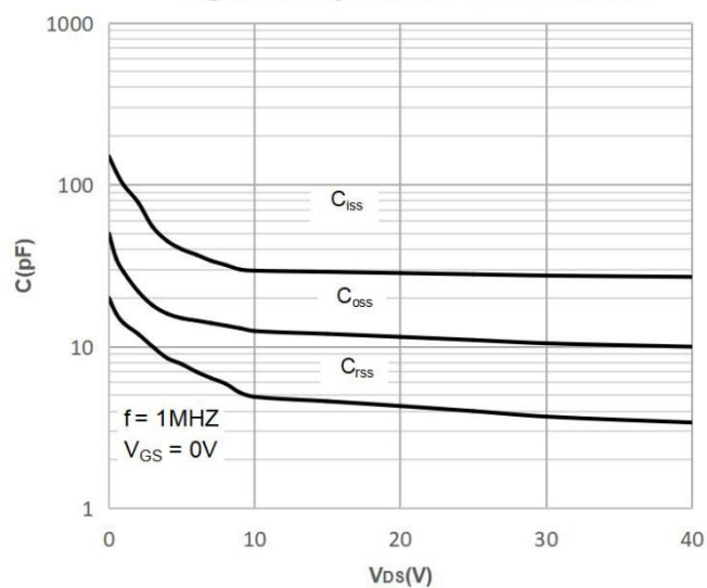
Figure 6: Capacitance Characteristics
