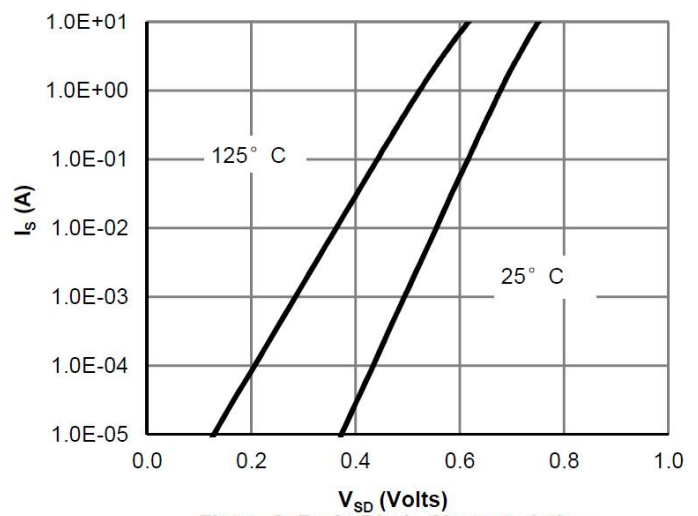
Figure 6: Body-Diode Characteristics
