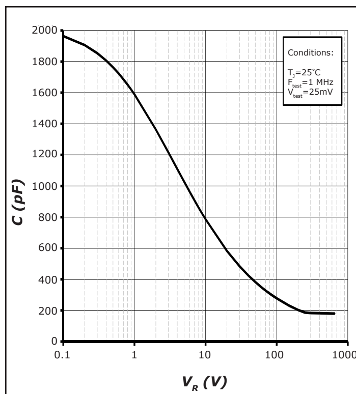
Figure 6. Typical Capacitance vs. Reverse Voltage
