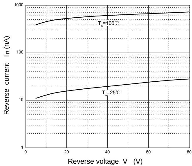
Figure 2: Reverse characteristics
