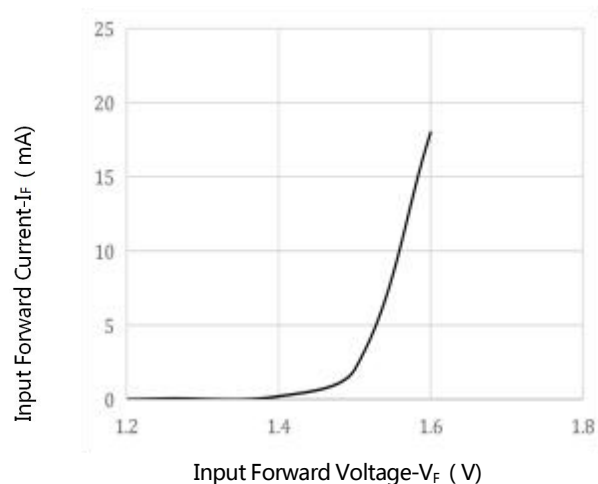
Fig.16 Input Forward Current vs Forward Voltage
