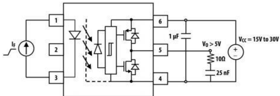
Figure 21 I_{FLH} Test Circuit
