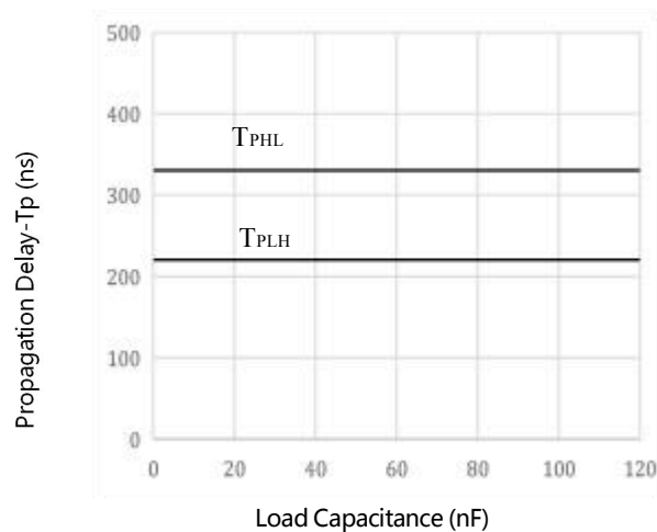
Fig.14 Propagation Delay vs. Load Capacitance
