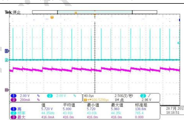
图 4, LEDs 短接 ( CH2: Drain CH3:Iout)
