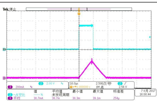
图 6, PWM 调光(100Hz/0.1%) (CH2:PWM CH3:Iout)
