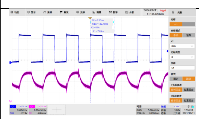
图8: 12Vin/8LEDs (CH1:V DRAIN CH4:I OUT )
