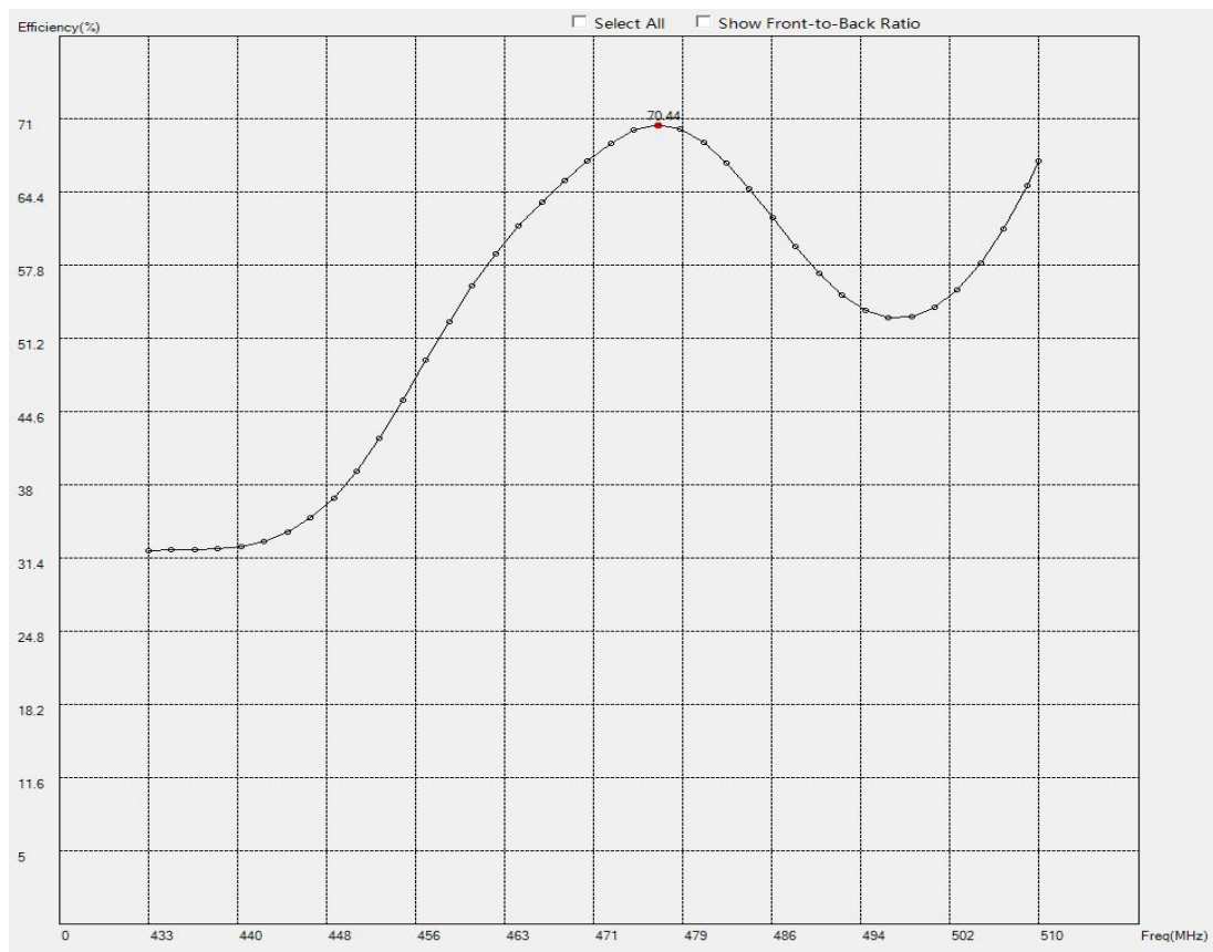
Efficiency (%/bend)
