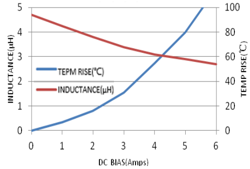
FSA0420-4R7MT
