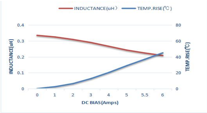
AFE141265SR33MBT
