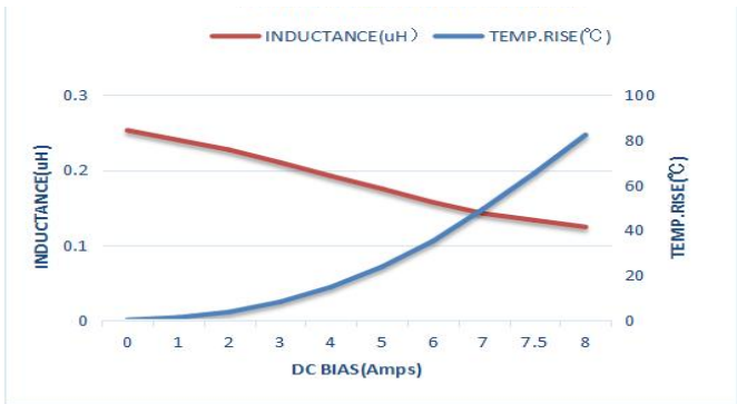
AFE141207SR24MBT
