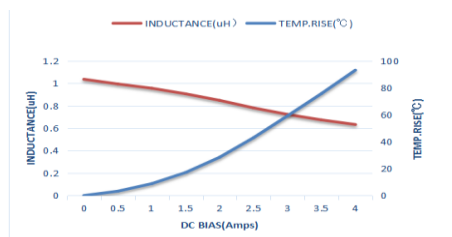
AFE160808S1R0MBT
