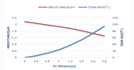
AFE160808S2R2MBT
