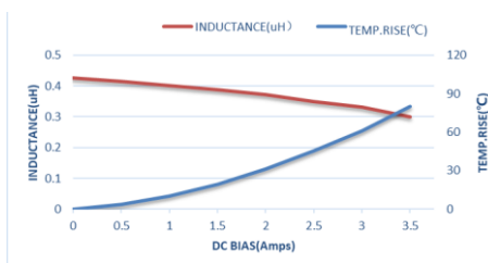
AFE160808SR22MBT
