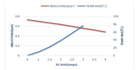
AFE160808SR68MBT
