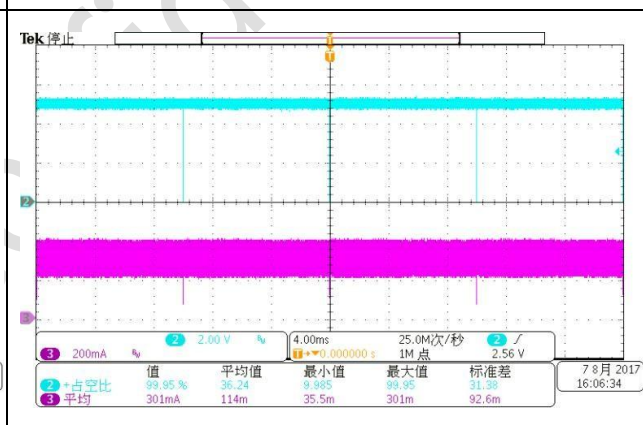
图 10, PWM 调光(100Hz/100%) (CH2:PWM CH3:Iout)
