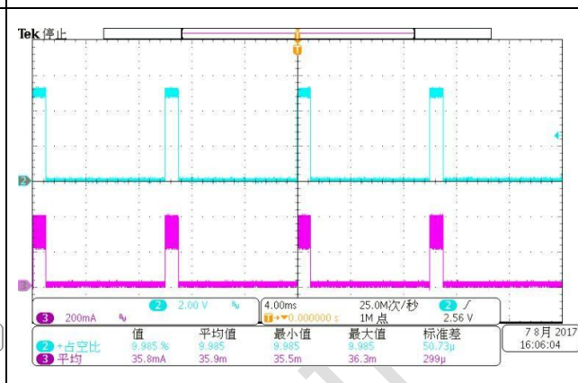
图 8, PWM 调光(100Hz/10%) (CH2:PWM CH3:Iout)
