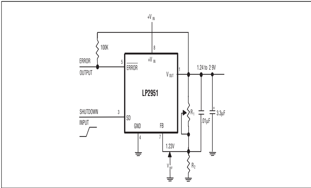
Figure 2. Adjustable Regulator
