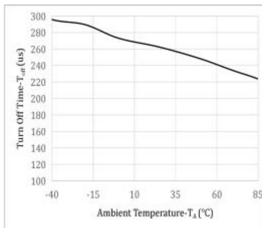
Fig.6 Turn Off Time vs. Ambient Temperature Characteristics
