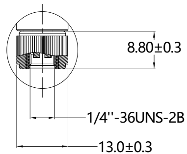
RF SMA-Male DETAIL A SCALE 2:1
