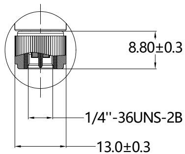
SMA-Male DETAIL A SCALE 2:1
