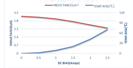
AFE201210S100MBT
