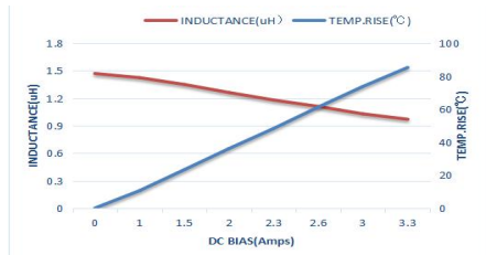
AFE201208S1R5MBT
