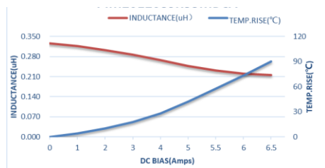
AFE201208S1R0MBT
