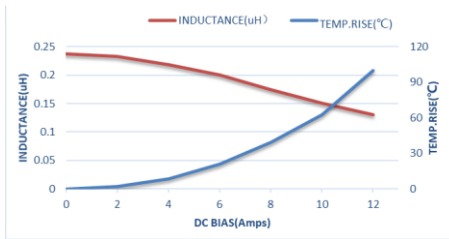
AFE201212SR24MBT
