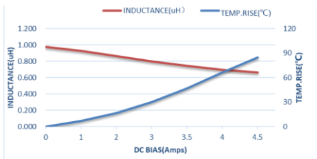
AFE201208S1R0MBT
