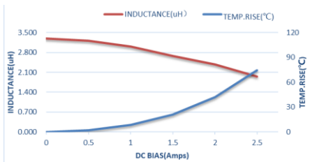
AFE201212S3R3MBT
