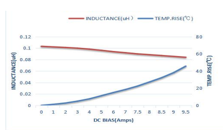
AFE201210SR10MBT
