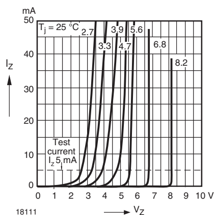
Fig. 14 - Breakdown Characteristics
