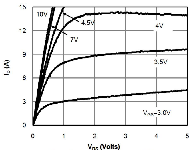
Figure 1: On-Region Characteristics
