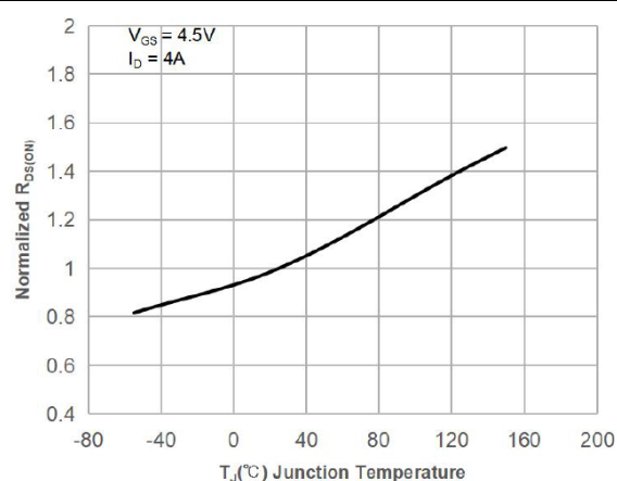
Figure 6: Normalized on Resistance vs Junction Temperature
