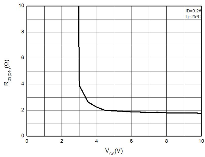
Figure13: on-Resistance vs. Gate to Source
