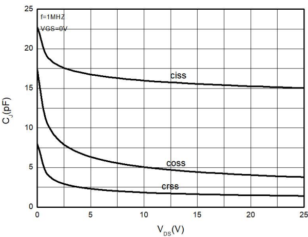
Figure4: Capacitance Characteristics
