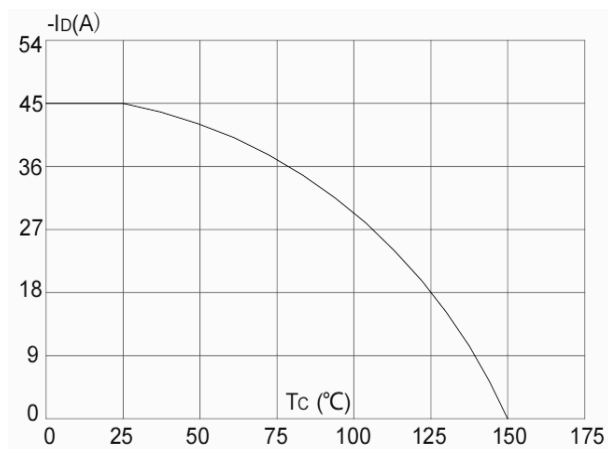
Figure 5: Current De-rating
