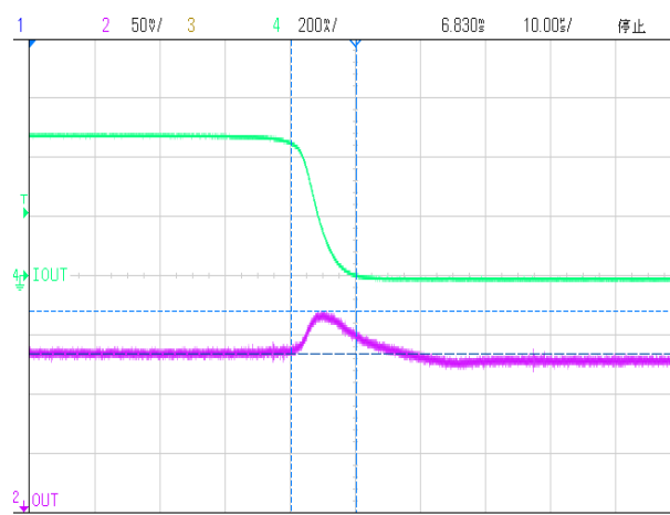
Load Transient(500mA to 1mA t=10us)
