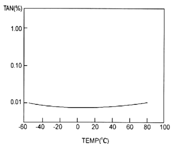
损耗角正切值与温度的关系 Connections between the dissipation factor and the temperature
