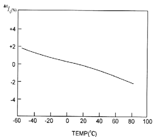
容量变化率与温度的关系 Connections between the capacitance change rate and the temperature
