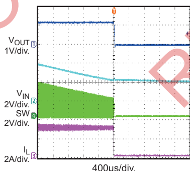
V_{IN} Shut down with 3A Load
