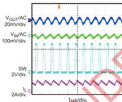
Input and Output Ripple
