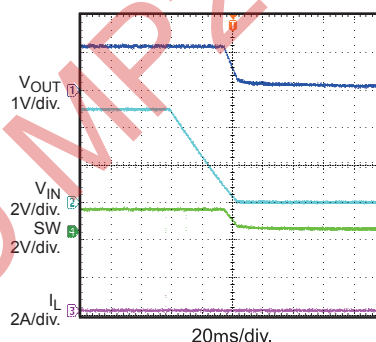
V_{IN} Shut down without Load
