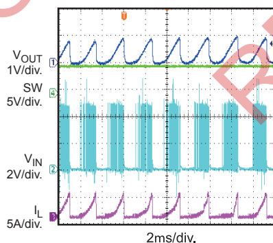
Short Circuit
