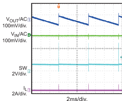
Input and Output Ripple
