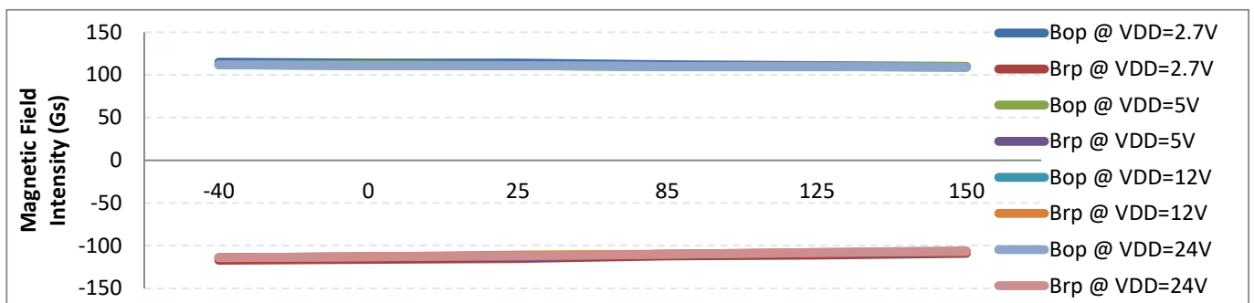
Figure.9 MT8962-Plus Magnetic Characteristics (BOP & BRP) vs. V_{DD} @ Temperature=25°C
