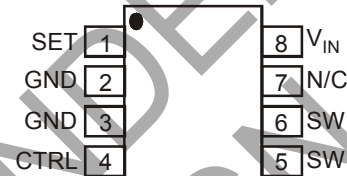
MSOP-8EP
