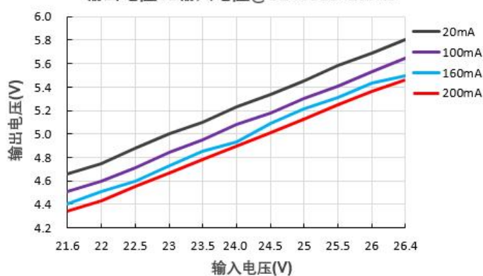
输出电压Vs输入电压@B2405LS-1WR3
