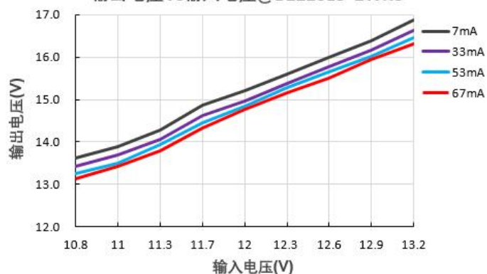
输出电压Vs输入电压@B1215LS-1WR3
