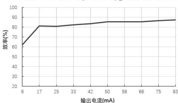
效率Vs输出电流(Vin=12V)@B1212LS-1WR3
