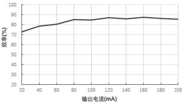
效率Vs输出电流(Vin=24V)@B2405LS-1WR3
