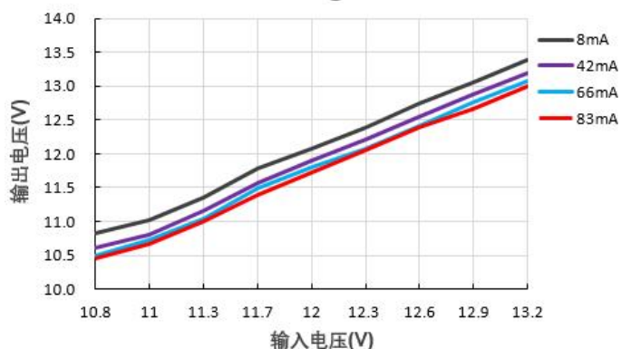
输出电压Vs输入电压@B1212LS-1WR3
