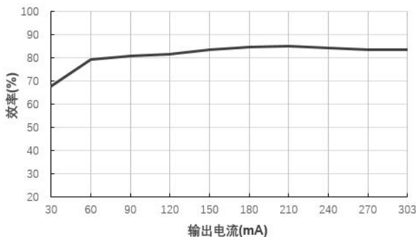
效率Vs输出电流(Vin=12V)@B1203LS-1WR3
