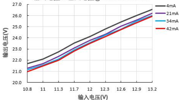
输出电压Vs输入电压@B1224LS-1WR3
