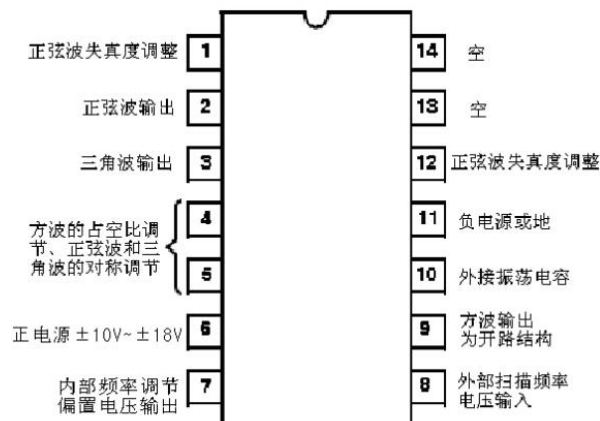
DIP-14/SOP-14/TSSOP-14
