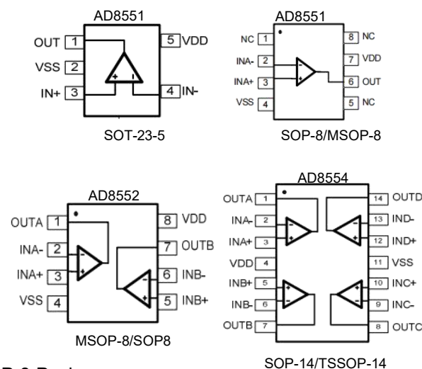
Figure 1. Pin Assignment Diagram
