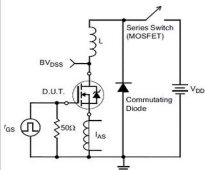
Figure 18 Unclamped Inductive Switching Test Circuit
