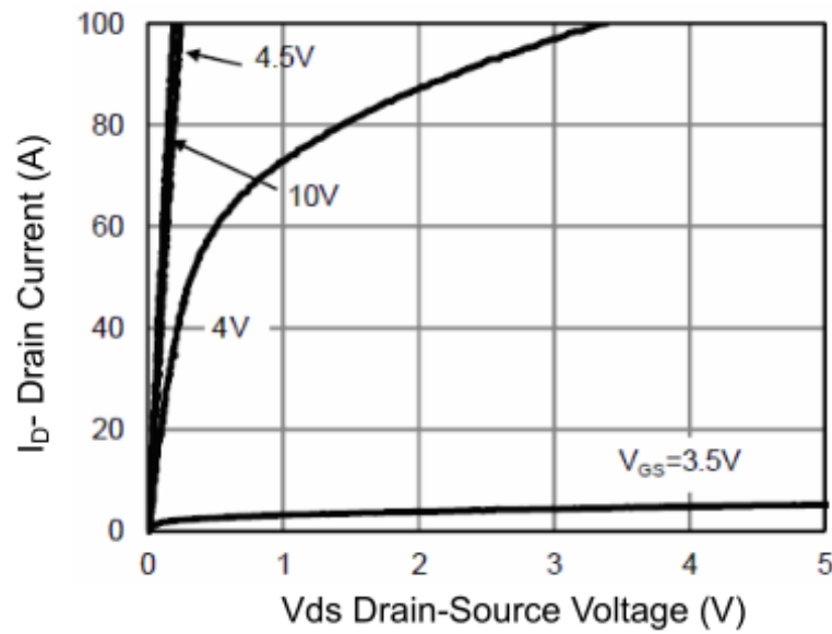
Figure 1 Output Characteristics
