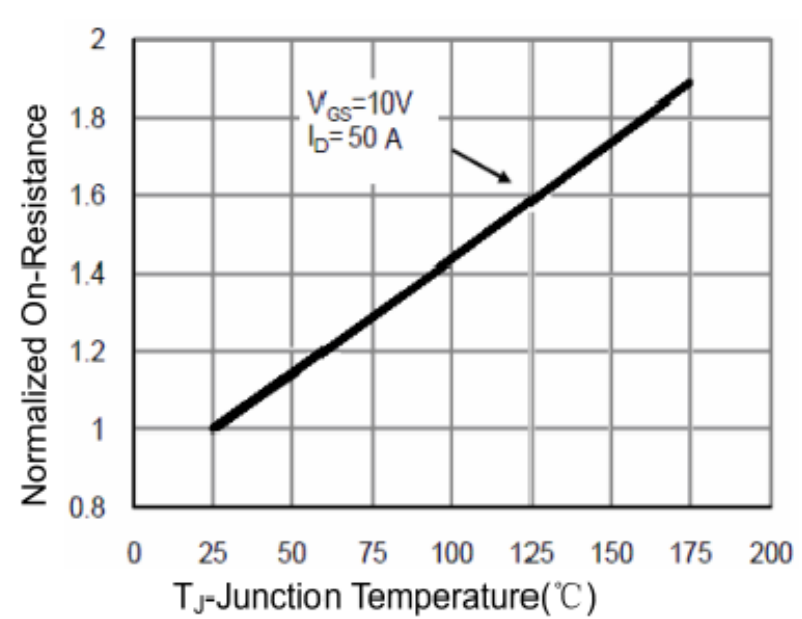
Figure 4 R_{DS(on)} -Junction Temperature
