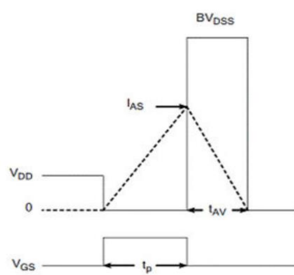
Figure 19 Unclamped Inductive Switching Waveform
