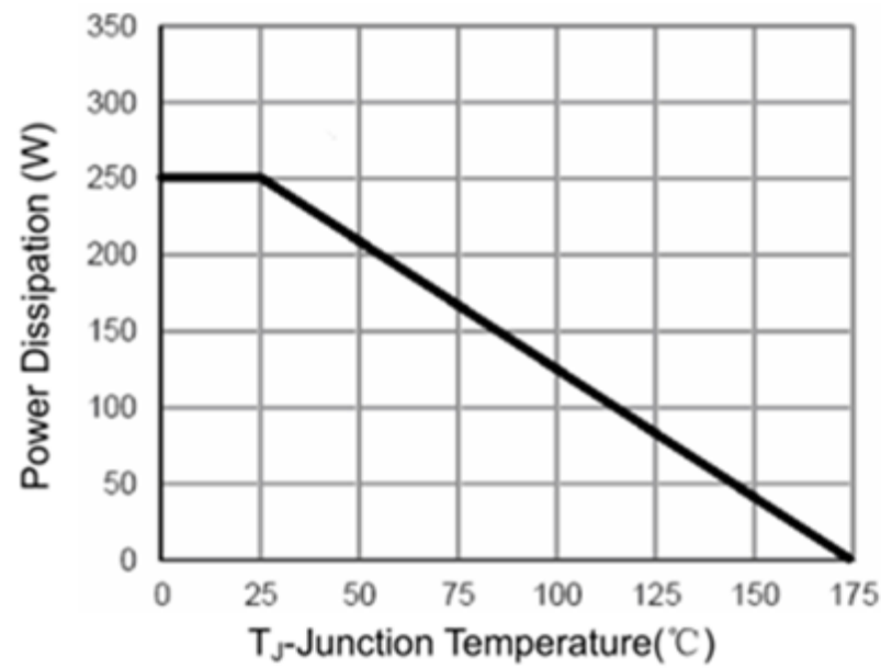
Figure 9 Power De-rating
