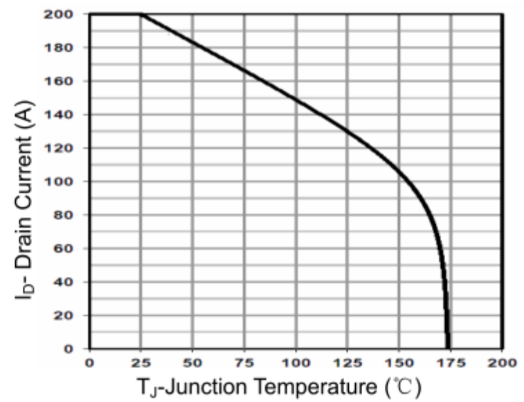
Figure 10 Current De-rating
