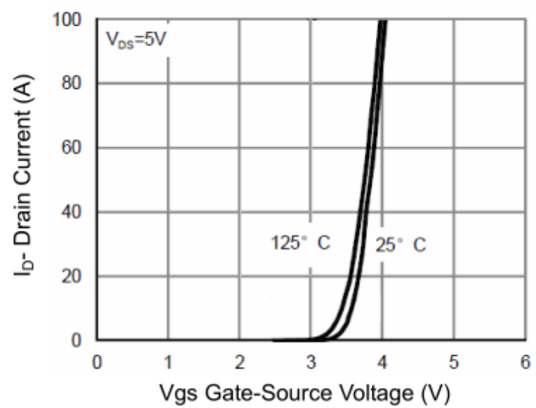
Figure 2 Transfer Characteristics
