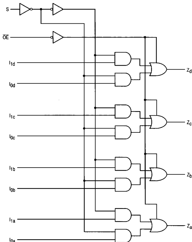
LOGIC DIAGRAM
