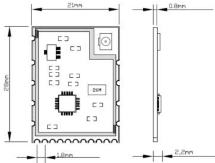
Figure 1: Module size
