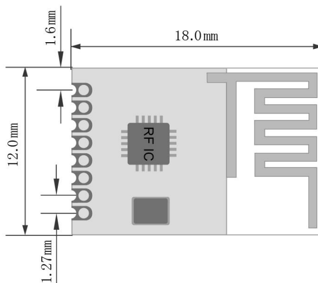
Figure 1: DL-Si24R1-A
