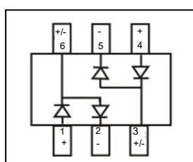
Equivalent Circuit
