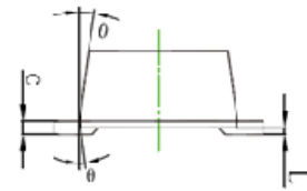
Package outline : SOD-523
