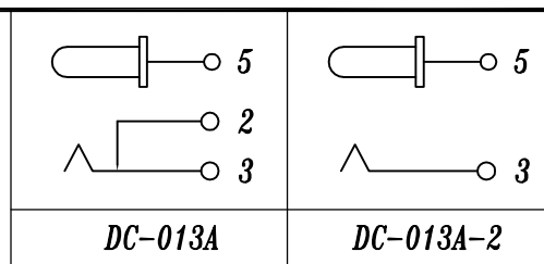
SCHEMATIC
