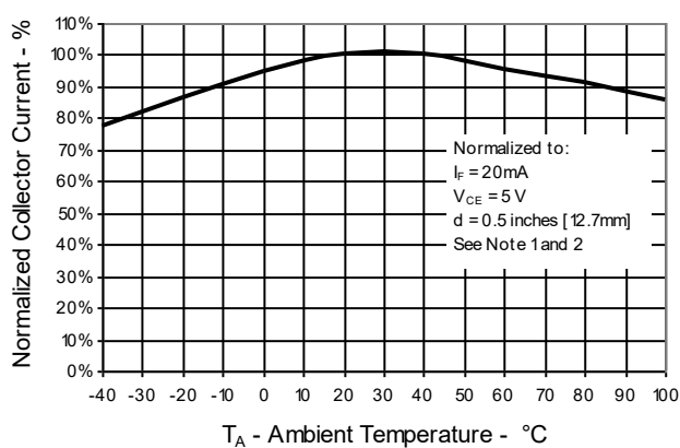
Normalized Collector Current Vs Ambient Temperature
