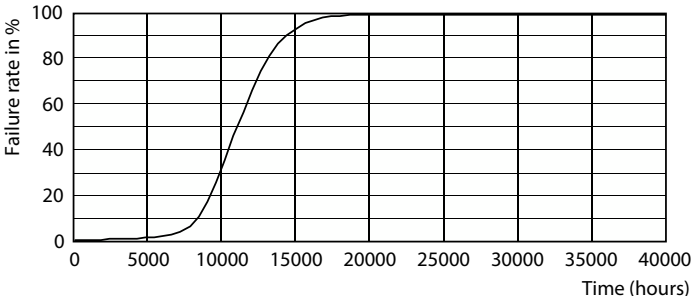
Life Expectancy Diagram - ESS LEDBulb 5W E27 6500K 230V 1CT/12 CN
