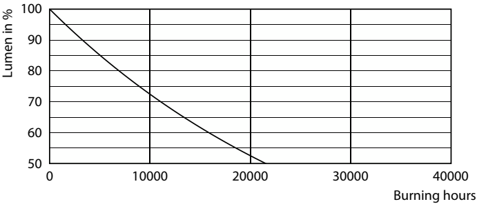
Lumen Maintenance Diagram - ESS LEDBulb 5W E27 6500K 230V 1CT/12 CN
