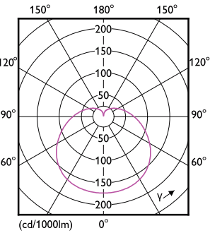
Light Distribution Diagram - ESS LEDBulb 5W E27 6500K 230V 1CT/12 CN
