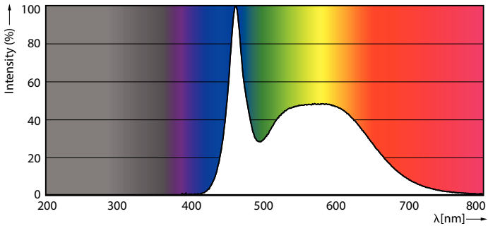
Spectral Power Distribution Colour - ESS LEDBulb 5W E27 6500K 230V 1CT/12 CN
