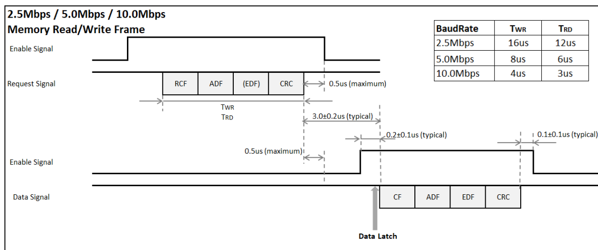
Figure 5: Timing Characteristics of Enable, Request, and Data Signals for Memory Access
