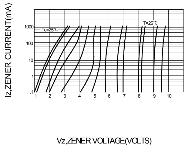
FIG.9 – ZENER VOLTAGE VERSUS ZENER CURRENT V_Z = 82 \text{ THRU } 200 \text{ VOLTS}
